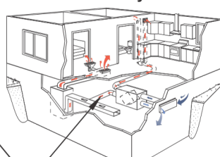
Motorized spring return damper (Highly Recommended)
