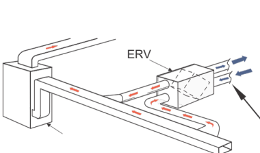
Furnace Return Air-duct Connection
