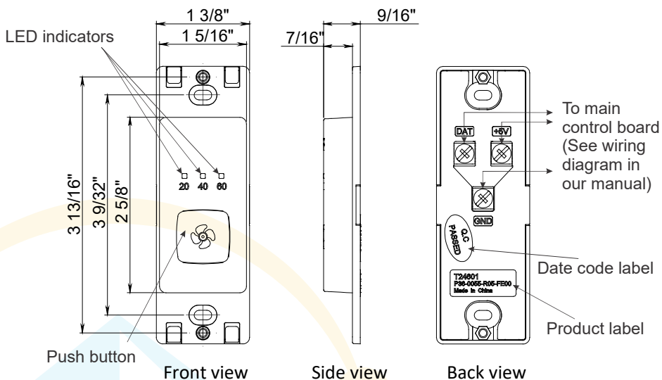
Fig 1.1 dimensional data
