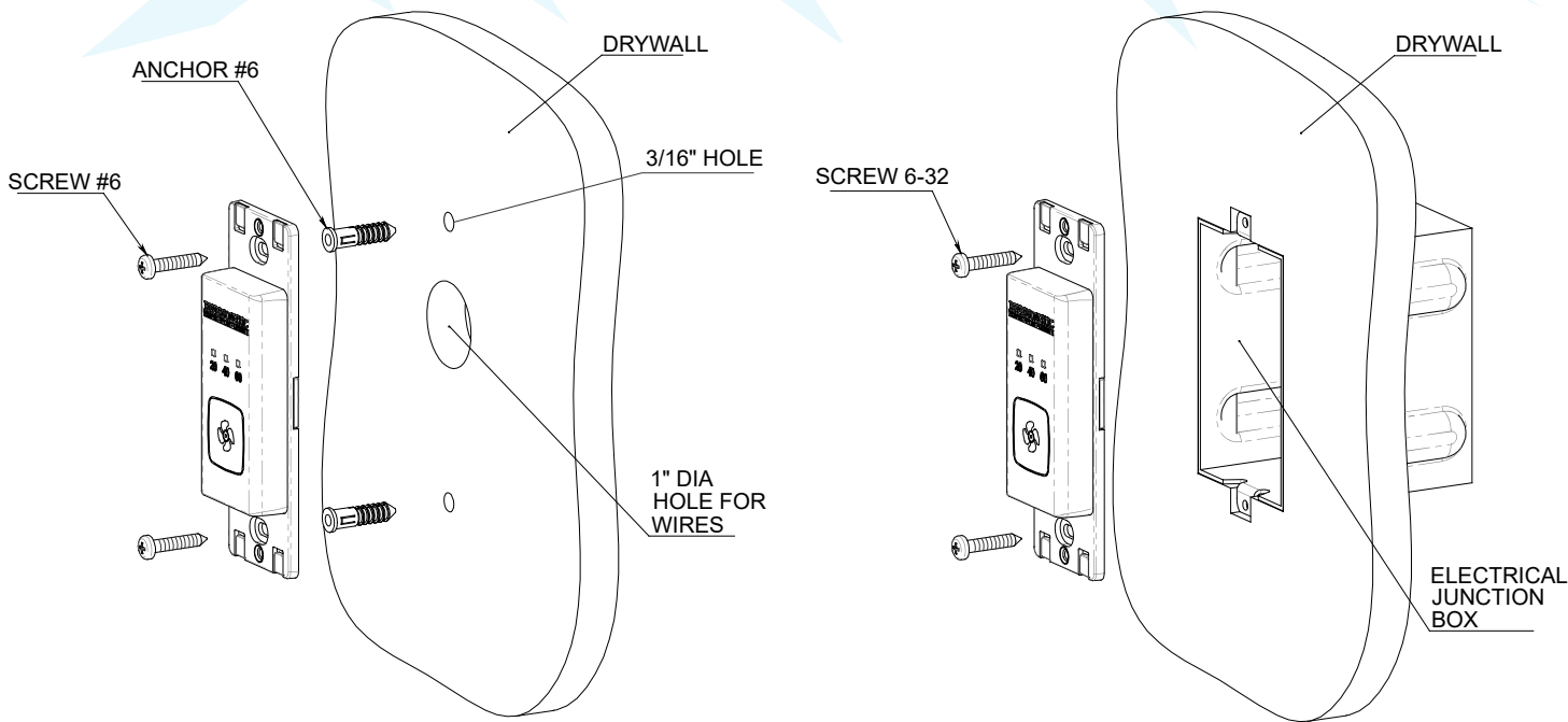
Fig 2.1 Installation on drywall
